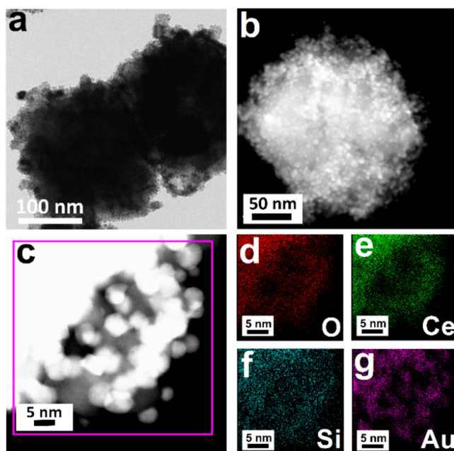
Figure 4. TEM (a) and HAADF-STEM (b) images of \text{o-CeO}_2@\text{SiO}_2@\text{c-CeO}_2/\text{Au} nanocomposites. (c) HAADF-STEM image of the edge on an \text{o-CeO}_2@\text{SiO}_2@\text{c-CeO}_2/\text{Au} nanoparticle. (d–g) Elemental mapping images of oxygen, cerium, silicon, and gold on the region shown in (c).
